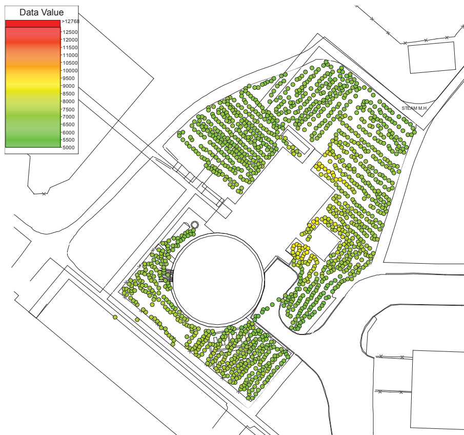
Figure 8: Gamma Walkover
